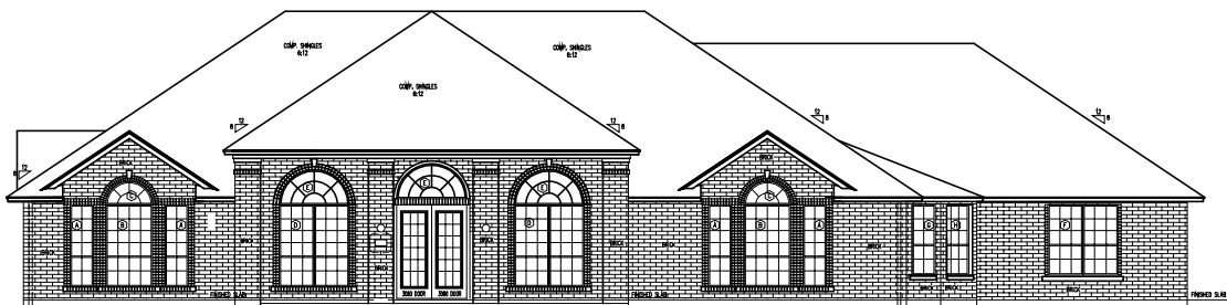
① FRONT ELEVATION
